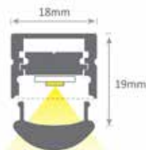
Profile
